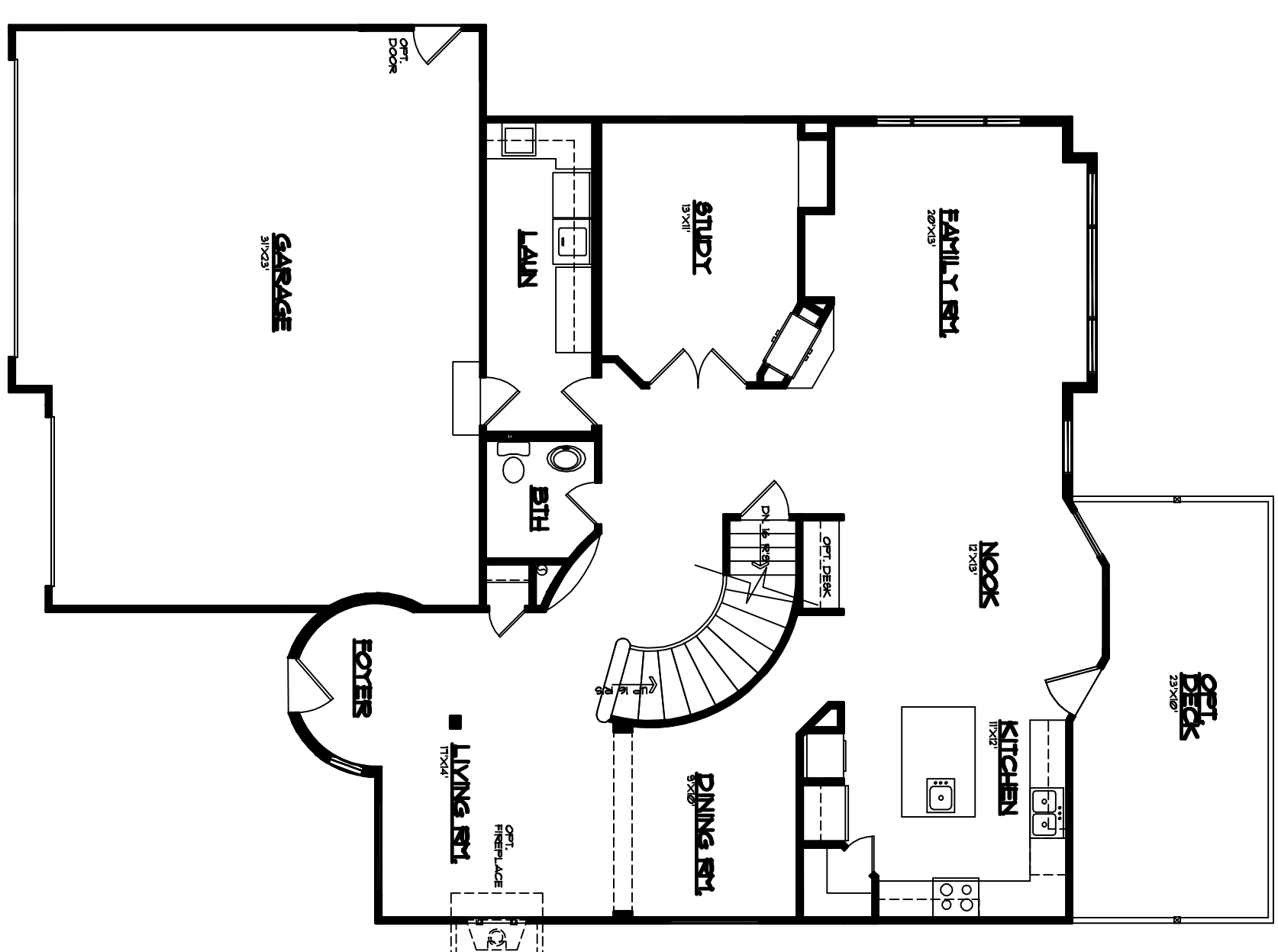
MODEL 3200 MAIN LEVEL 30' 0" x 37'
