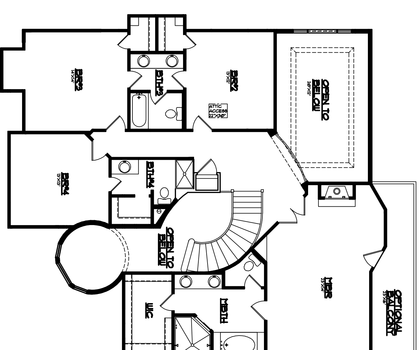
MODEL 3200 UPPER LEVEL 30' 0" x 37'
