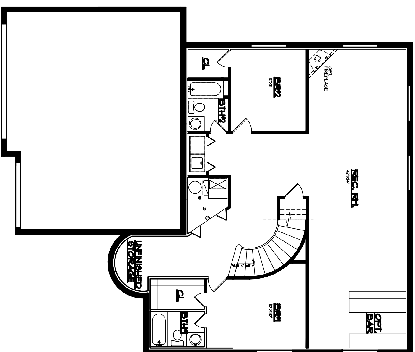
MODEL 3200 LOWER LEVEL 30' 0" x 37' NOTE: OPT. BASEMENT FINISH
