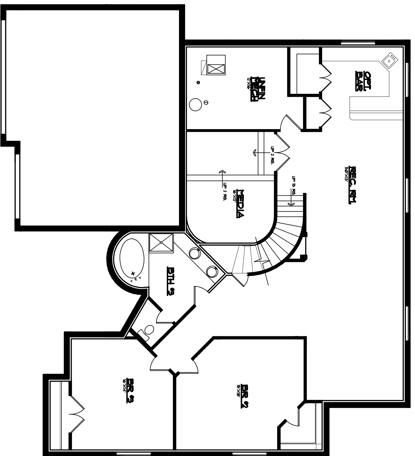
MODEL # 2323 LOWER LEVEL NOTE: OPT. BASEMENT FINISH
